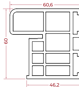
PASSIVEDOOR / WARMDOOR
